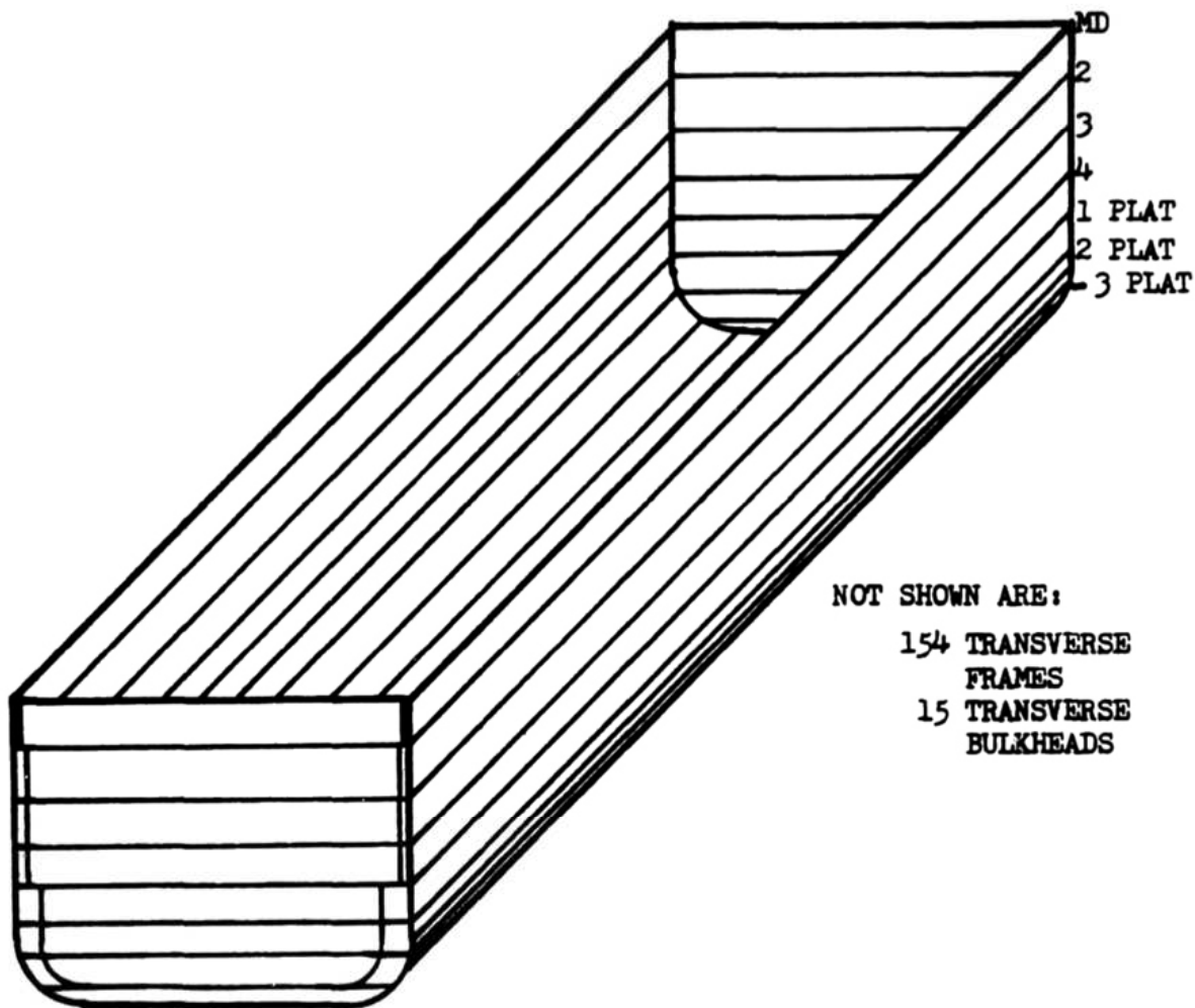
FIGURE 14.1. A DIAGRAM OF THE SHIP MODEL USED FOR THE ECONOMIC IMPACT STUDY
