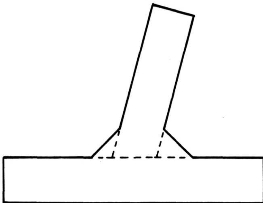
FIGURE 6.6. ANOTHER SKEWED FILLET WELDED TEE JOINT
