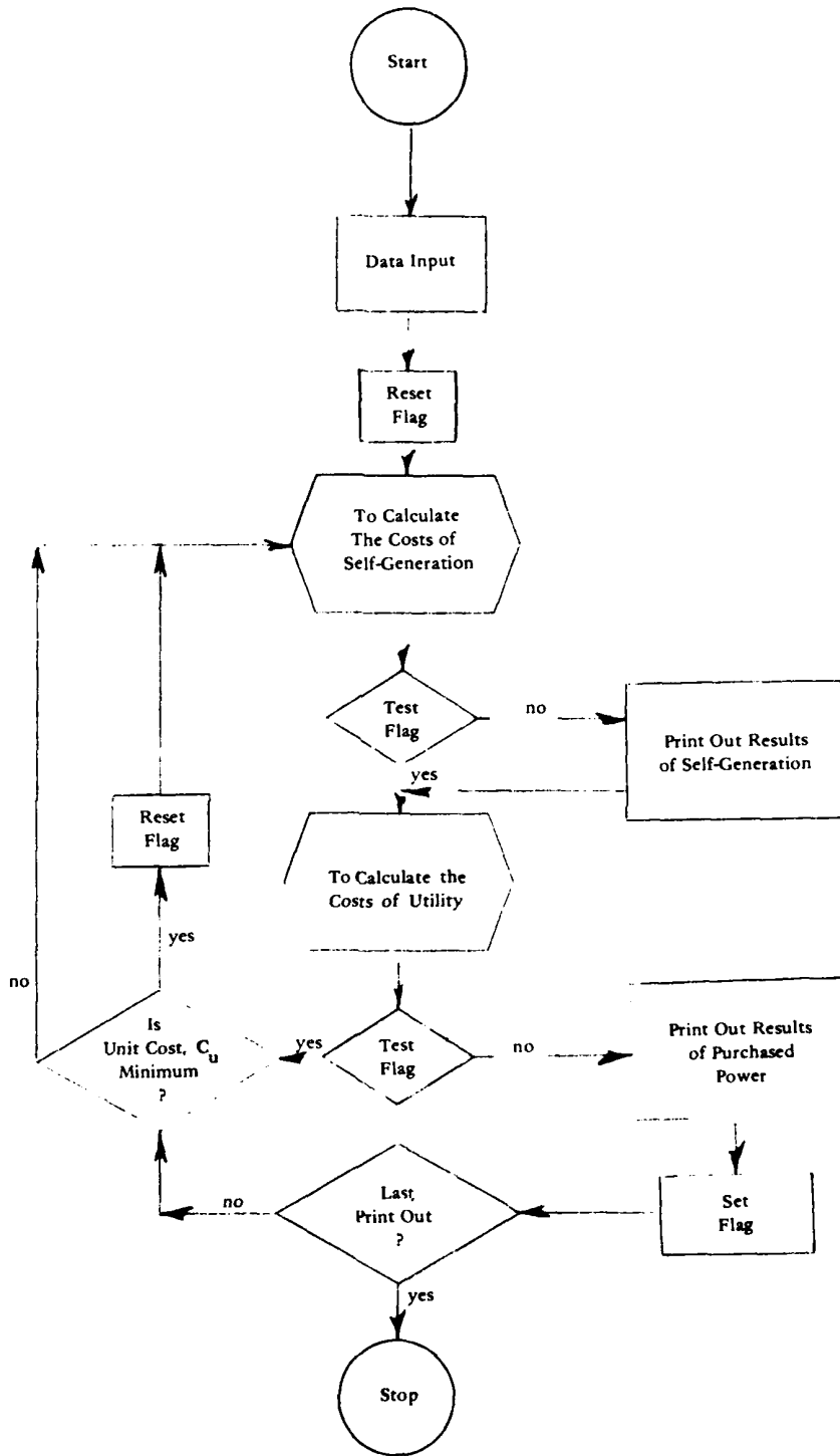
Figure 5. Flow chart of computer program.
